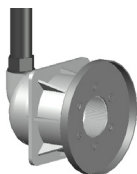
PZA-WCS-NG + PZA-FLEX-S * Niche for UF-DVA Built-in length: 145 mm Hole size: 1.5" BSP Conduit connection: 3/4" BSP
