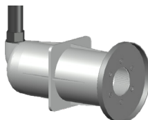
PZA-WC-NG + PZA-FLEX-S * Niche for UF-DVA Built-in length: 262 mm Hole size: 1.5" BSP Conduit connection: 3/4" BSP
