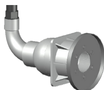
PZA-WCS-NG + PZA-FLEX-NG * Niche for UF-DVA Built-in length: 225 mm Hole size: 1.5" BSP Conduit connection: 3/4" BSP
