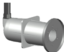
PZA-WC-NG + PZA-FLEX-S * Niche for UF-DVS Built-in length: 262 mm Hole size: 1.5" BSP Conduit connection: 3/4" BSP
