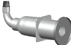
PZA-WC-NG + PZA-FLEX-NG * Niche for UF-DVS Built-in length: 345 mm Hole size: 1.5" BSP Conduit connection: 3/4" BSP
