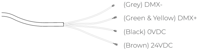
RGBW Light Cable Connection
