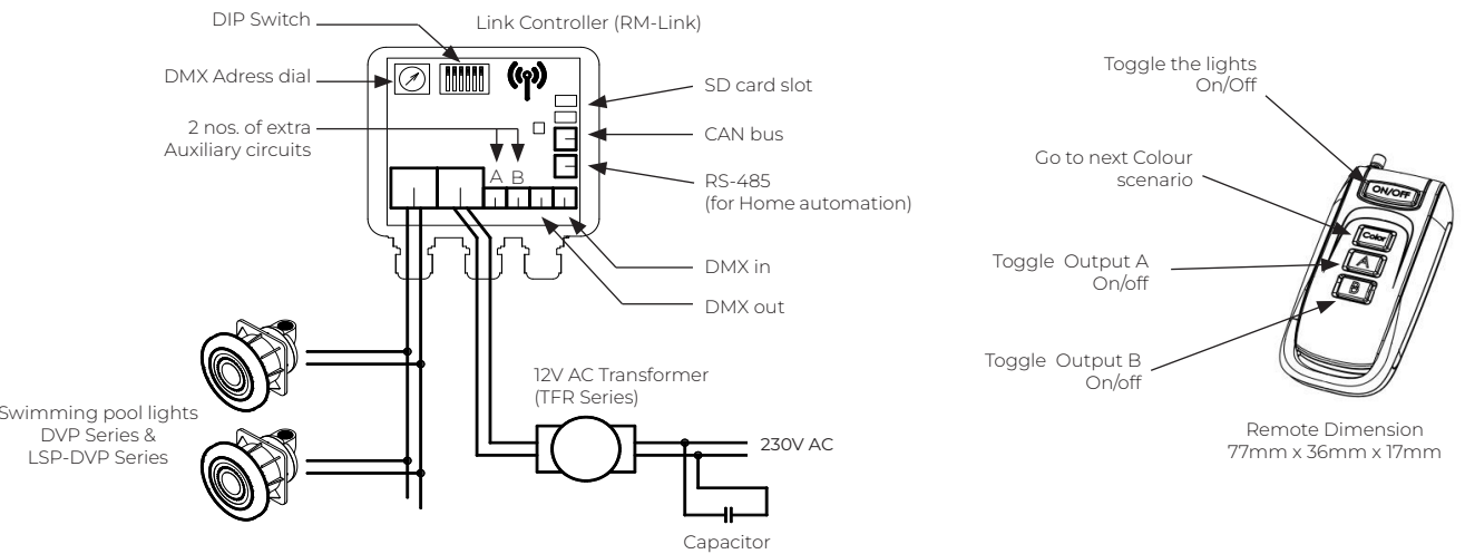
Link Touch - RGB(W) * for RGB or RGBW lights
