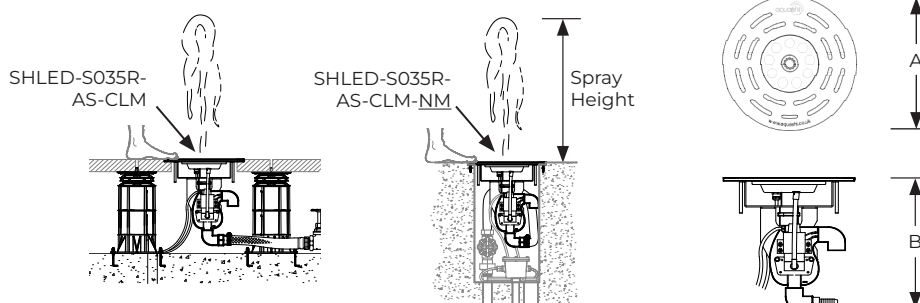
Round Slab Hanger LED Light with Column Jet Nozzle Aquaswitch
